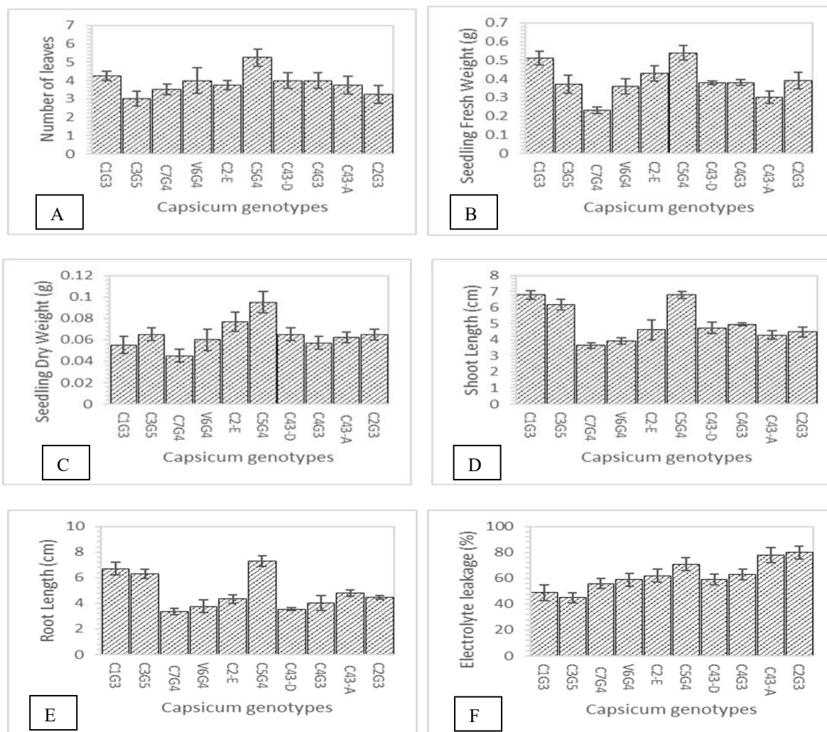
Figure Effect of heat stress (40°C) on (A) number of leaves, (B) seedling fresh weight (g), (C) seedling dry weight (g), (d) shoot length (cm) (e) root length (cm) and (f) electrolyte leakage (%)
